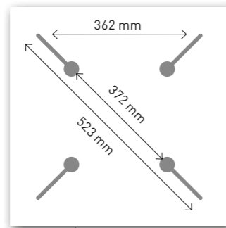
Fixing 2 The secure mounting system using grooves milled on one side allows the tops to be fixed to all conventional bases without drilling. Groove length 200 mm. > Special bolts provided.
