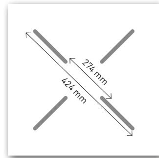
Fixing 3 The Eco fixing system consists of a 10 mm wide rail, in which we fix the bases using special 6x12 screws. > Screws included. > Only available for 10mm Carino.
