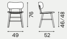
Lounge
