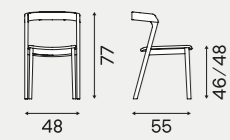
Chair/Sedia
